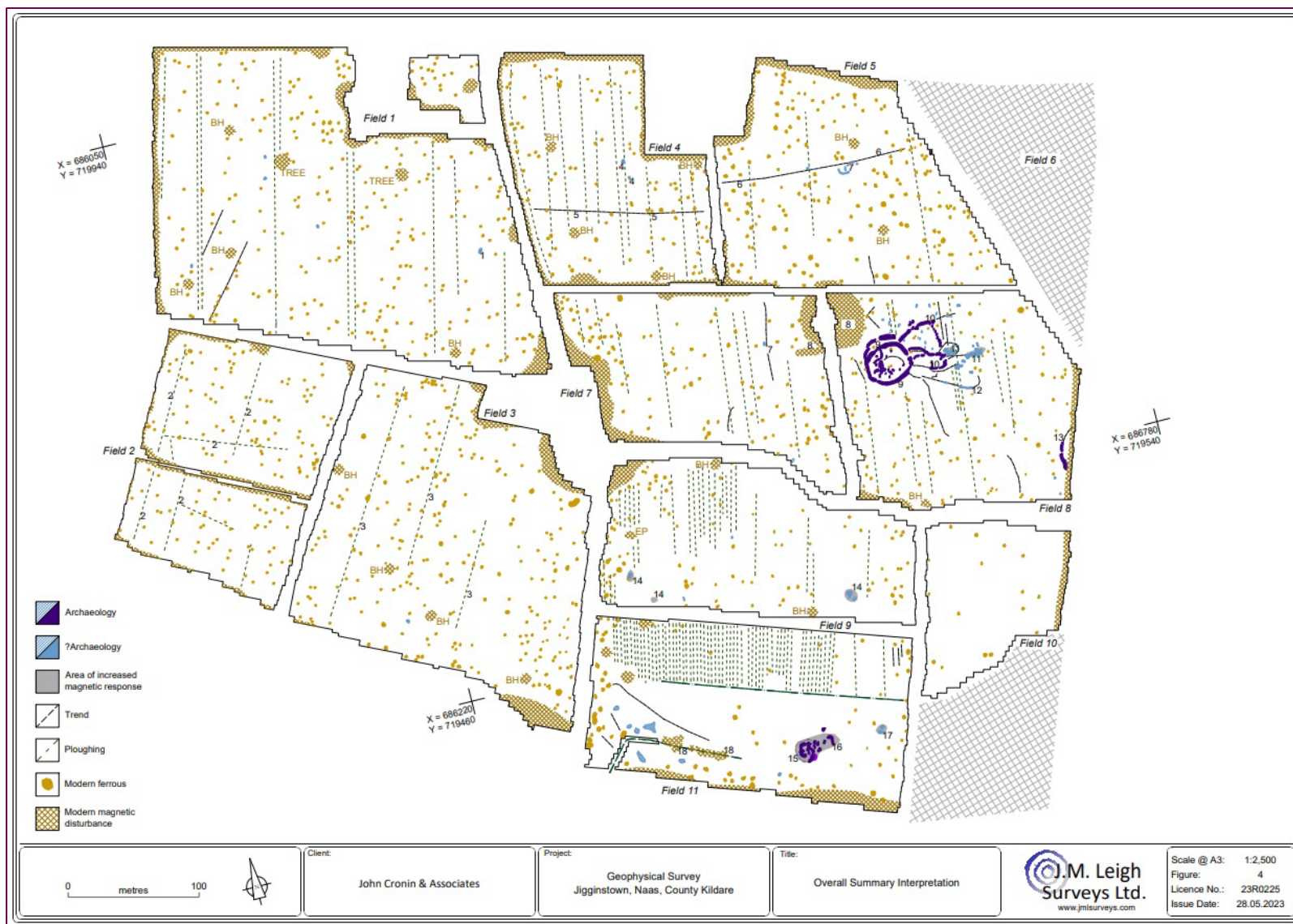
Figure 10.1: Interpretative image showing results of geophysical surveys (23R0105 and 23R0225)
